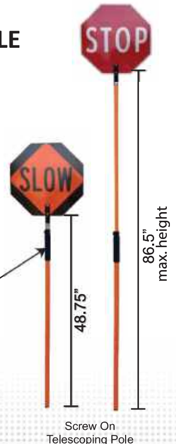
Screw On Handle Pole Height Adjustment Mechanism SSP-P-83
