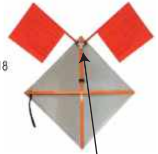
Metal Bracket is riveted to roll-up cross brace
